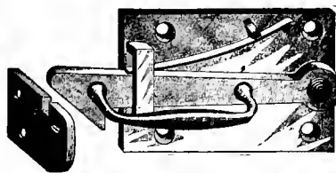
Figs. 2558-2559. Spring Latch and Keeper for Baggage-car Sliding-door.
